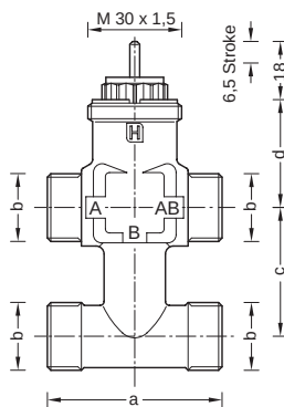
Three-way valve with integral bypass VZ42
