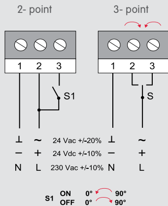
electrical diagram
