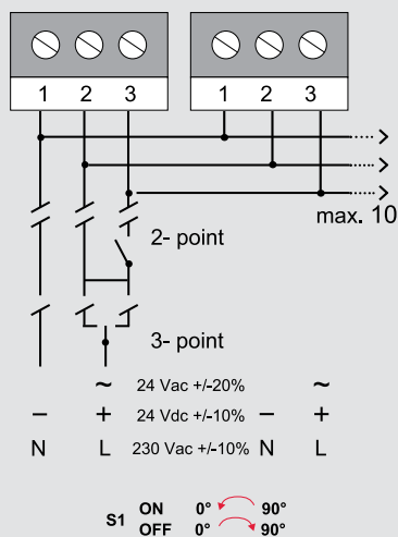
parallel connections
