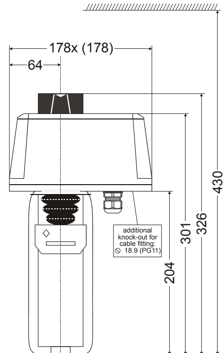
Fig. 2. ML6421B (dimensions in mm)
