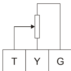
auxiliary potentiometer
