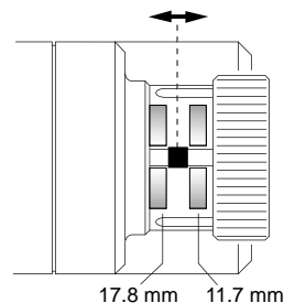
Fig. 9. Movement of actuator stem
